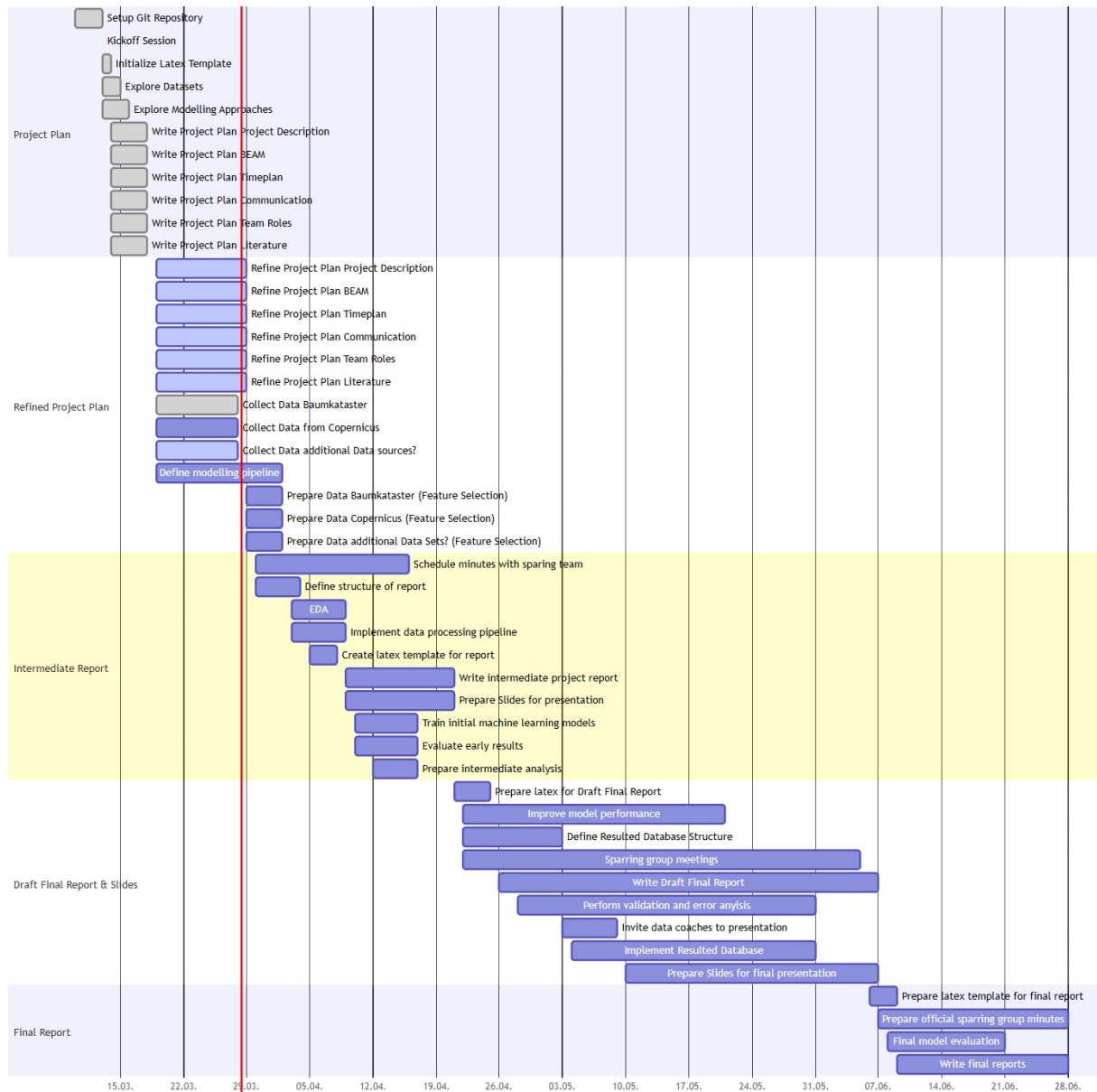
Figure 2: GANTT Diagramm
